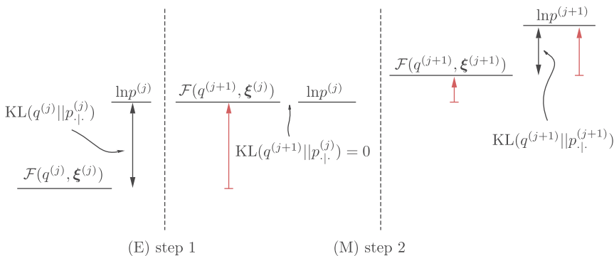
The E-step adjusts q^{(j)} := q^{(j)}(\mathcal{X}^l) so that its KL divergence from p_{\cdot}^{(j)} := p(\mathcal{X}^l | \mathcal{X}; \xi^{(j)}) becomes zero. The M-step maximizes with respect to \xi . We used p^j to denote the evidence function.
